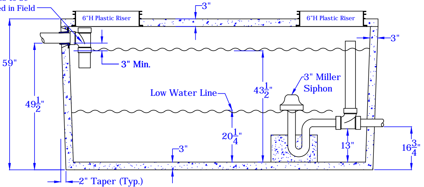
AA Section of 1250 Gallon Siphon Tank No Scale
