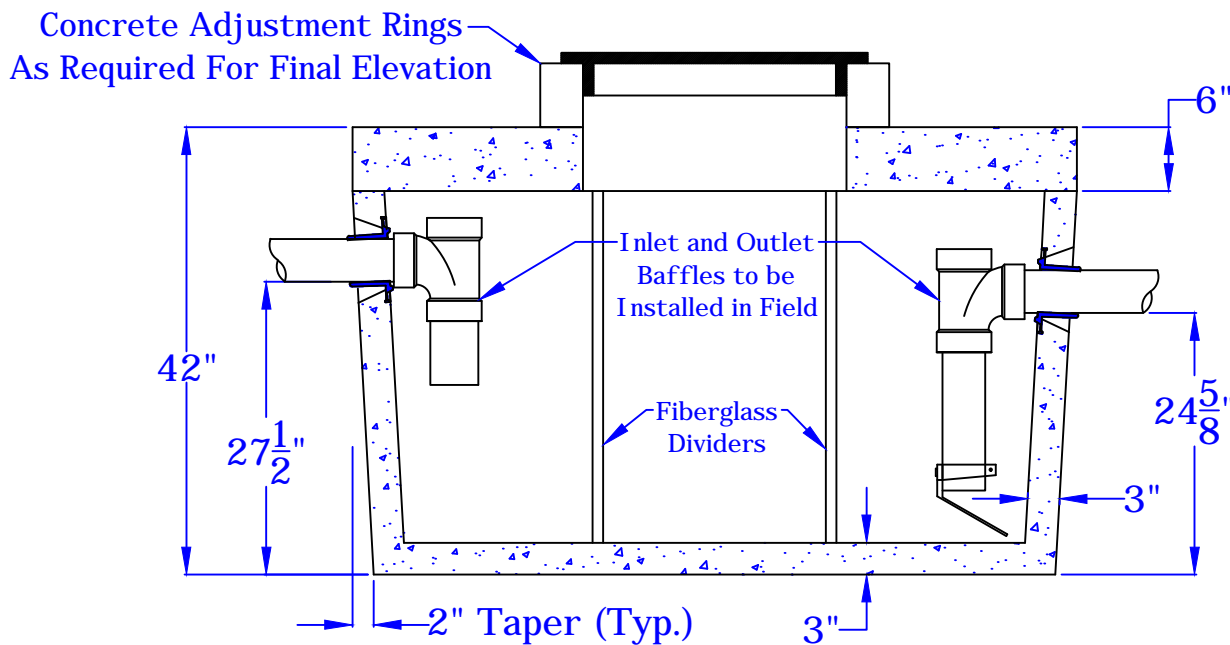
AA Section of 250 Gallon Oil/Water Separator Not To Scale
